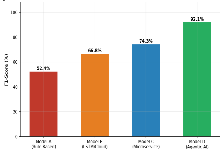
Figure 2. Anomaly Detection and Decision Accuracy (F1-Score %) across Architectural Models. Model D Demonstrates Statistically Significant Accuracy Gains through Unified Agentic Reasoning
