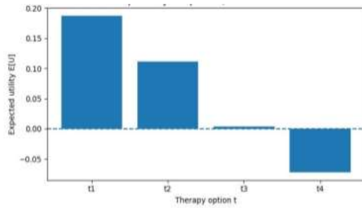
Figure 6. Utility Comparison; Chosen t^* = t_1
