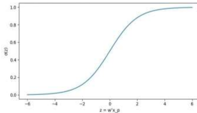
Figure 5. Sigmoid Mapping from Linear Score to Response Probability
