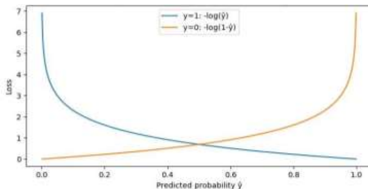
Figure 8. Binary Cross-Entropy Loss as a Function of Predicted Probability
